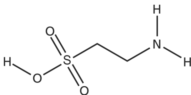
Figure 1. Taurine structure.
