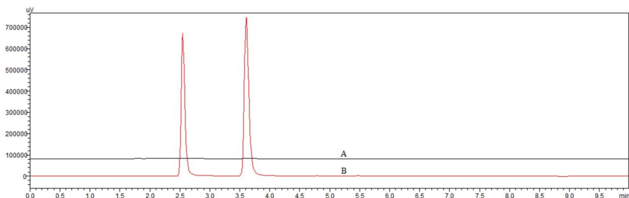
Figure 2. Typical chromatograms of blank [A], rosuvastatin and ezetimibe [B].
