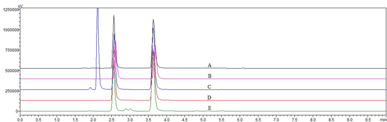
Figure 3. Typical Chromatograms of rosuvastatin and ezetimibe on acidic [A], alkali [B], oxidation [C], thermal [D] and photolytic [E] degradations.
