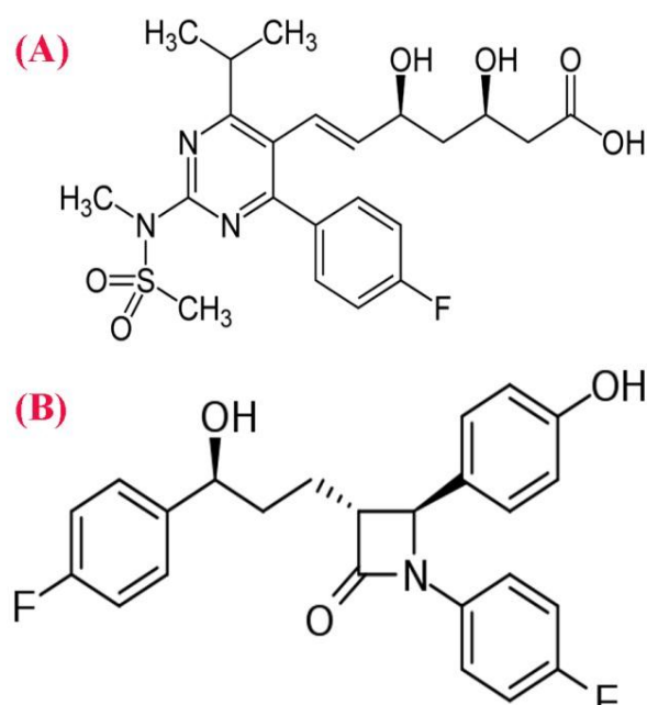
Figure 1. Chemical structures of rosuvastatin [A] and ezetimibe [B].
