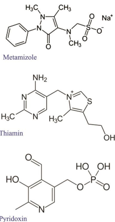
Figure 1. The chemical structure of Metamizole, Vitamin B 1 and Vitamin B 6 .
