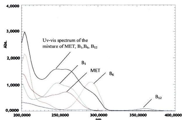
Figure 2. The overlay of UV spectra of Metamizole, Vitamin B 1 and Vitamin B 6 .
