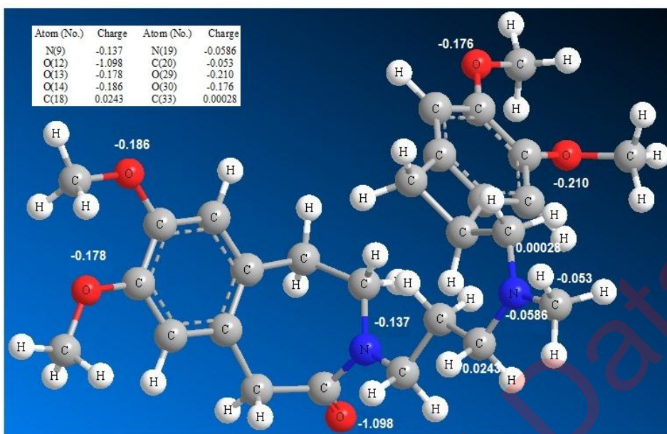
ESI 3. The charges of atoms of IH.
