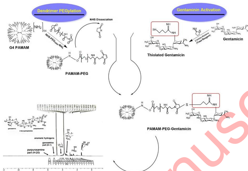
Figure 1. The schematic of the synthesis process of PAMAM-PEG 3400 -Gentamicin nanoparticles.
