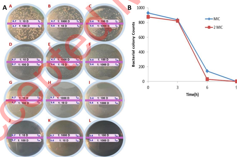
Figure 6. Time kill study assay. (A) The cultured plate at time 0 (A-C), 3h (D-F), 6h (G-I), and 9h (J-L) after incubation with MIC (~4.7 \mu g/ml) and 2MIC (~9.4 \mu g/ml) of PAMAM-PEG-Gentamicin. The dilutions of 1:10, 1:100 and 1:1000 were prepared and then Pour Plate was performed. (B) Time-kill study curves with P. aeruginosa . The concentrations of gentamicin used represent the respective MIC and 2MIC.
