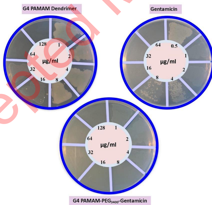
Figure 4. The evaluation of compounds minimum inhibitory concentration (MIC).
