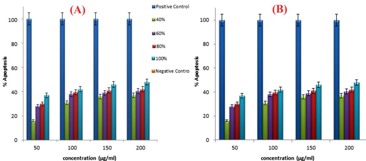
Figure 2. Apoptotic effect of O. cuspidatum methanolic fractions (40%, 60%, 80% and 100%) on PC-3 (A) and WEHI-164 cells (B) in 24 hours. The data represent the mean \pm SE of three independent experiments each in triplicate format ( p < 0.05 ).
