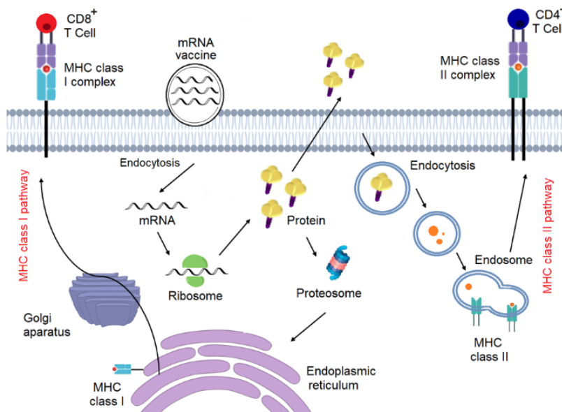
Figure 1. Mechanism of action of mRNA vaccines.
