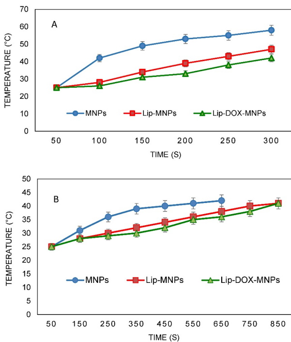
Figure 5. Magnetic heating curves for groups consist of magnetic nanoparticles (A) before in-vivo test under power of 1000 W and frequency of 405 kHz, (B) after injection in mice under power of 1000 W and frequency of 405 kHz. (The data represent mean \pm standard deviation)
