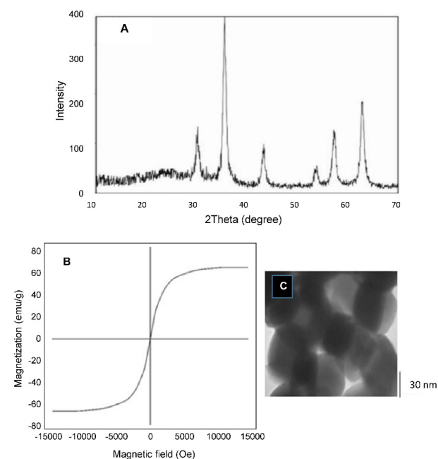
Figure 1. (A) X-ray pattern, (B) M-H curves of Fe 3 O 4 nanoparticles, (C) TEM image of Fe 3 O 4 particles.
