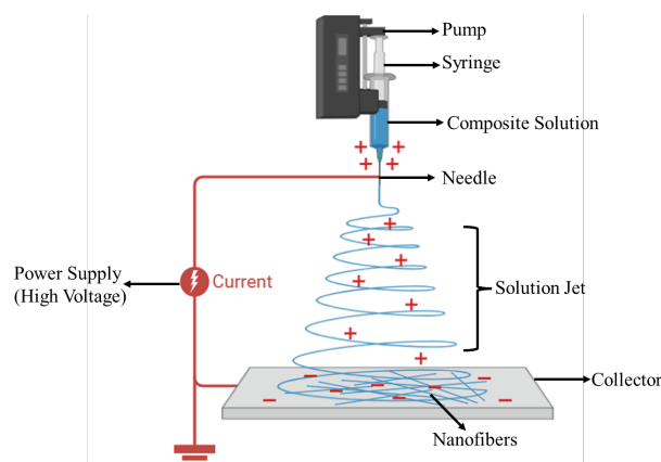
Figure 1. Development of nanofibers using electrospinning technique
