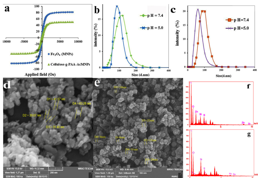
Figure 5. Magnetic properties of Fe_3O_4 and Cellulose-g-PAA-g-PACMNPs with magnetization values of about 81 and 50 respectively (a) Hydrodynamic diameters of Cellulose-g-PAA-g-PACZnO (b), Cellulose-g-PAA-g-PACMNPs (c), Surface morphology of Cellulose-g-PAA-g-PACZnO (d), Cellulose-g-PAA-g-PACMNPs (e) Semi-qualitative determination of elements on the surface of Cellulose-g-PAA-g-PACZnO (f) , Cellulose-g-PAA-g-PACMNPs (g) by SEM-EDX elemental analysis.
