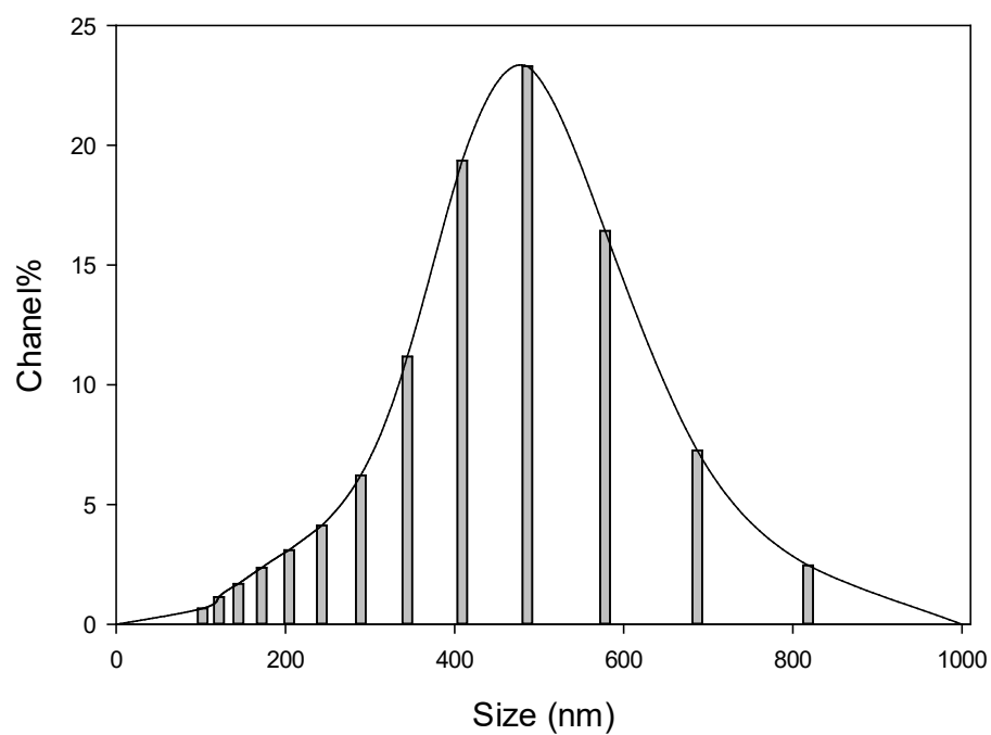
Figure S3. Dynamic light scattering, size distribution histogram, MS-NH 2
