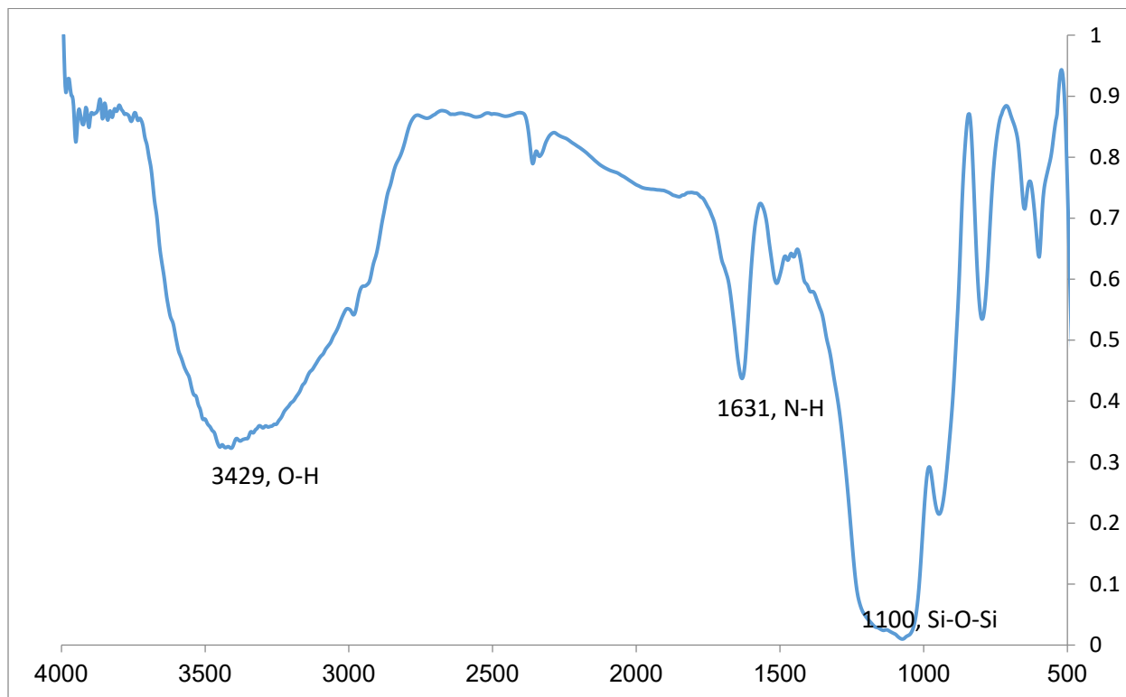
Figure S1. FT-IR spectrum of MSN-NH 2
