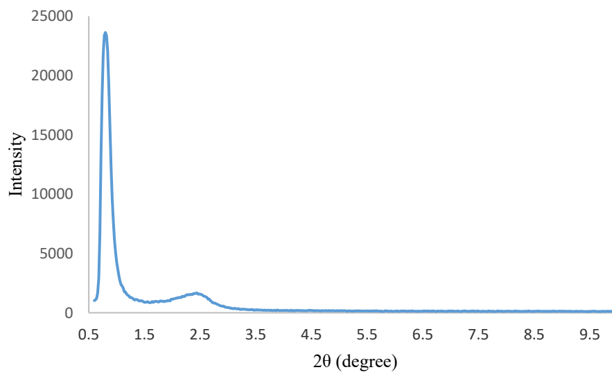
Figure S2. XRD patterns of MS-NH 2
