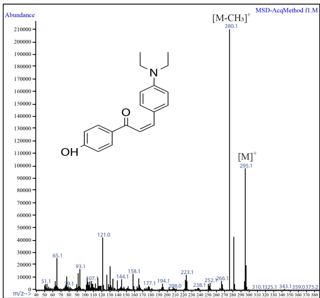
Figure S4. MS-EI spectrum of (Z)-3-(4-(diethylamino)phenyl)-1-(4-hydroxyphenyl) prop-2-en-1-one (Compound 3).
