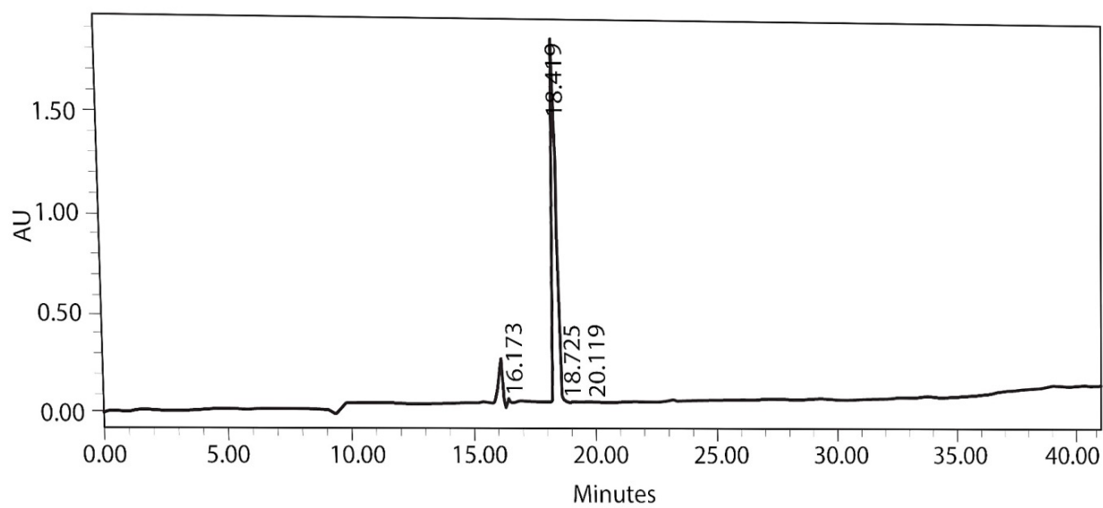
Figure S7. HPLC profile of DTPA[Ch-DE] 2 (Compound 6).
