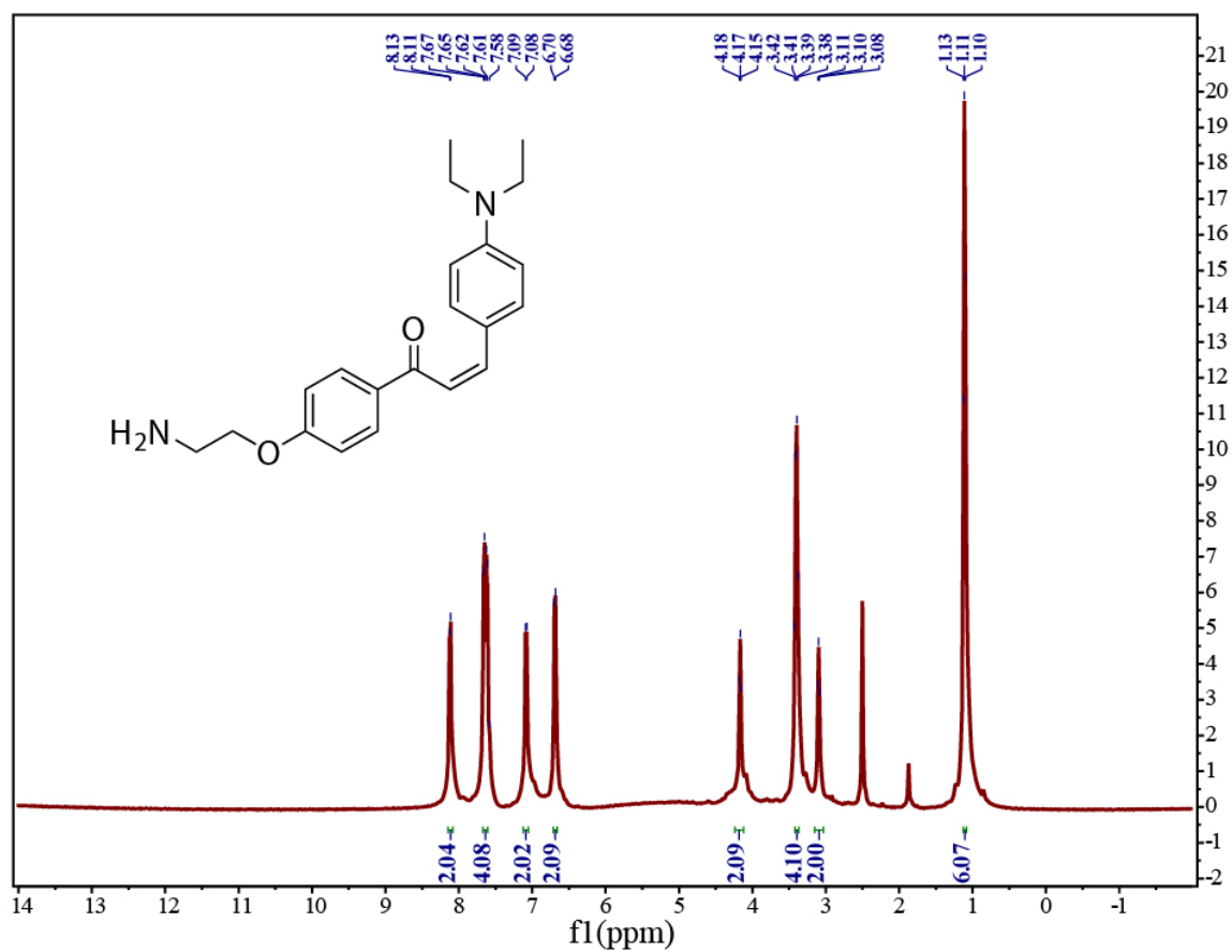
Figure S6. 1 H NMR spectrum (Z)-1-(4-(2-aminoethoxy) phenyl)-3-(4-(diethylamino) phenyl) prop-2-en-1-one (Compound 5).
