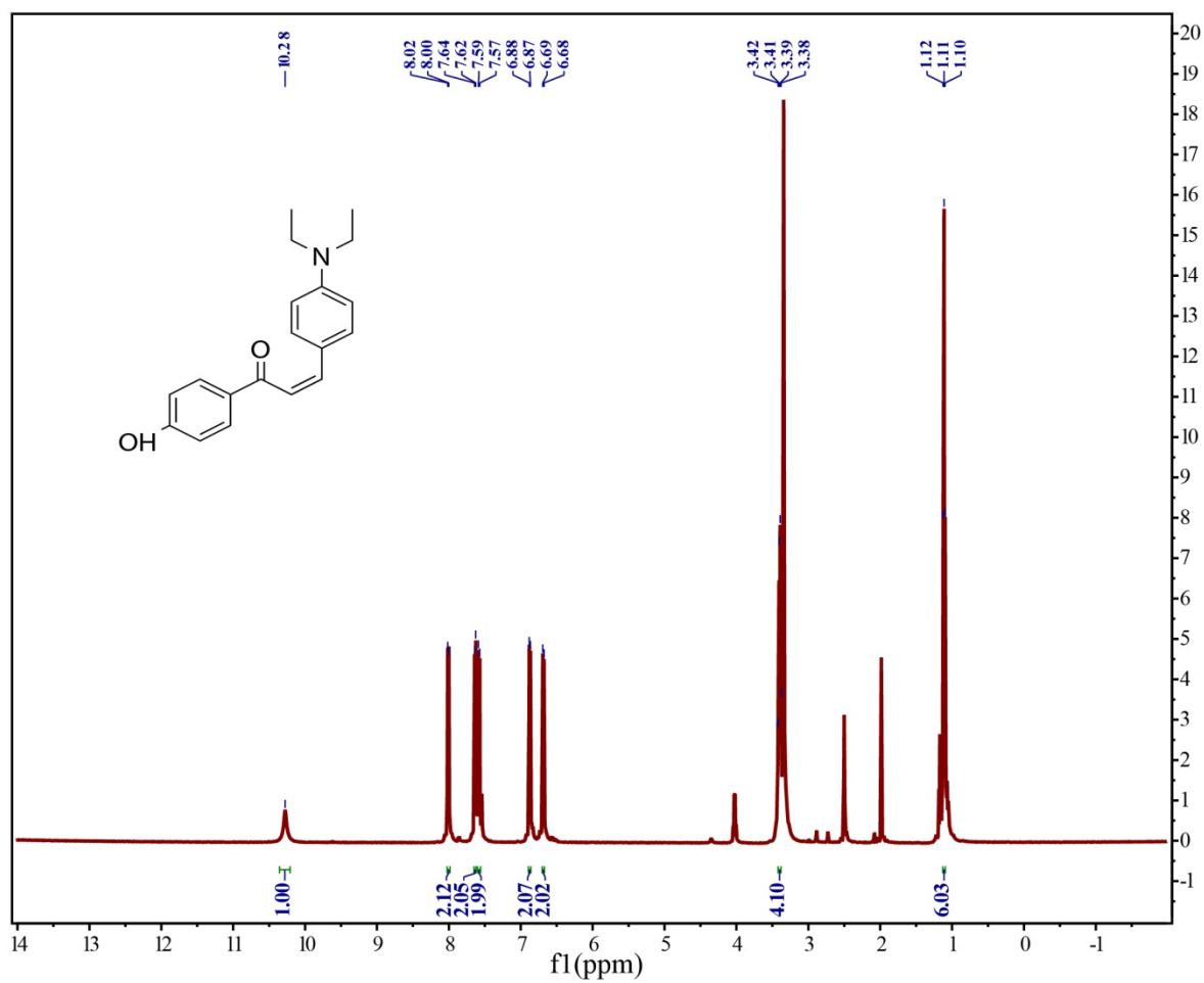
Figure S3. 1 H NMR spectrum of (Z)-3-(4-(diethylamino)phenyl)-1-(4-hydroxyphenyl) prop-2-en-1-one (Compound 3).
