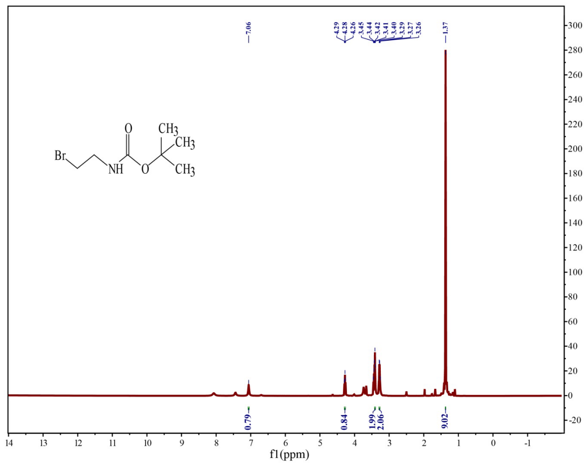
Figure S1. 1 H NMR spectrum of tert -Butyl 2-bromoethylcarbamate (Compound 1).
