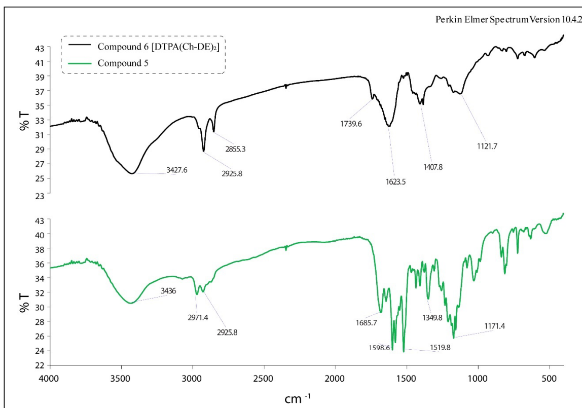
Figure S9. FT-IR spectrum of (Z)-1-(4-(2-aminoethoxy) phenyl)-3-(4-(diethylamino) phenyl) prop-2-en-1-one (Compound 5), and DTPA[Ch-DE] 2 (Compound 6).
