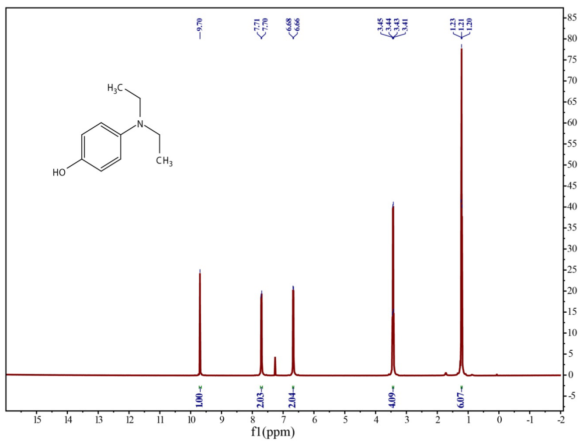
Figure S2. 1 H NMR spectrum of Para-diethylaminobenzaldehyde (Compound 2).
