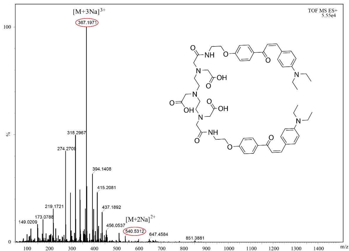
Figure S8. Mass spectrum of DTPA[Ch-DE] 2 (Compound 6).
