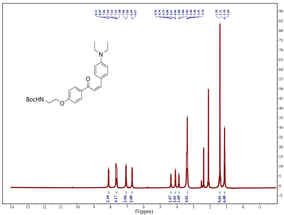
Figure S5. ^1\text{H} NMR spectrum (Z)-tert-butyl-2-(4-(3-(4-(diethylamino)phenyl)acryloyl)-phenoxy)ethyl carbamate (Compound 4).
